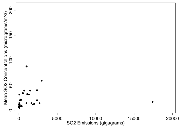
Figure 1 \text{SO}_2 Emissions and Mean \text{SO}_2 Concentrations, 1995
