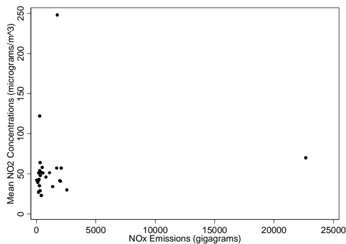
Figure 2 \text{NO}_x Emissions and Mean \text{NO}_2 Concentrations, 1995
